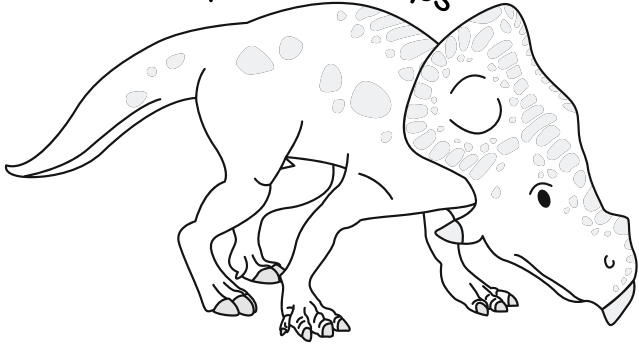
protoceratops
